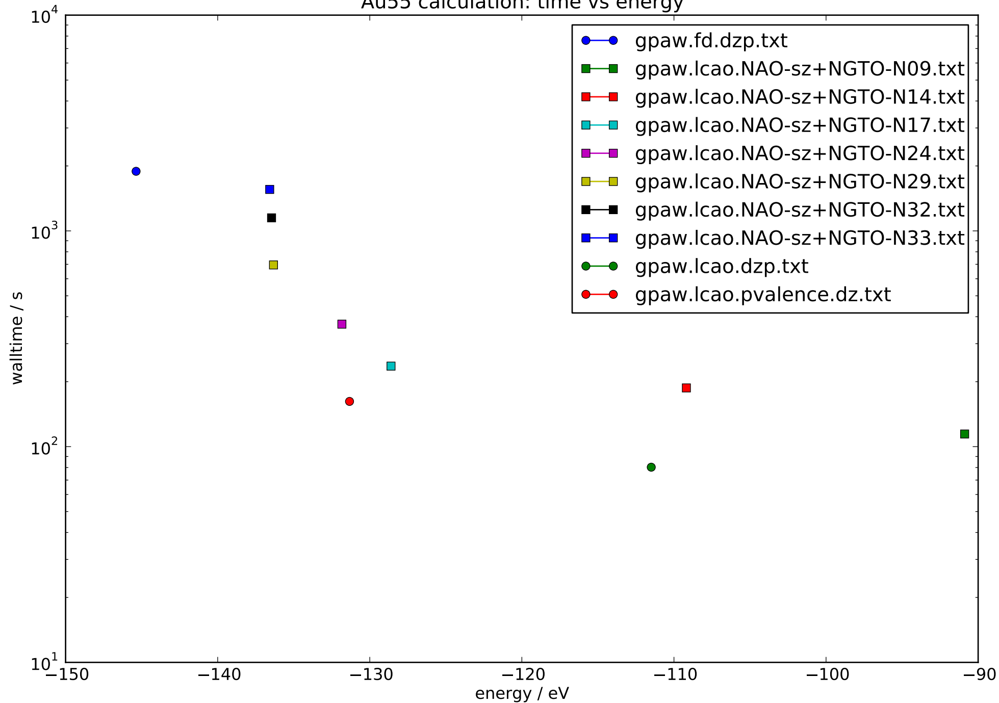
Au55 calculation: time vs energy
